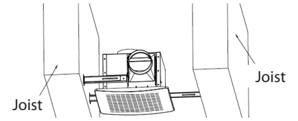
Joist Mounting Installation
