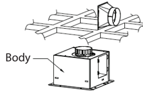
Wood Frame Installation
