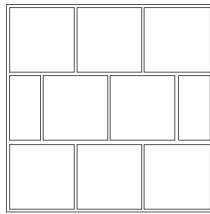
BRICK PATTERN 100 pcs. per 100 s/f 12 x 12 100% OR 400 pcs. per 100 s/f 6 x 6 100%
