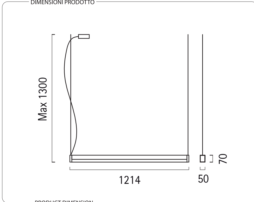
PRODUCT DIMENSION
