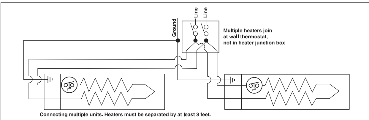
Figure 12 Connecting Multiple Units Left End Wiring 240 or 208 volt models only
