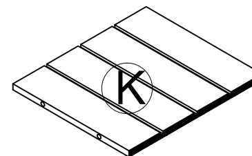
Bottom panel Panel base T9345096110
