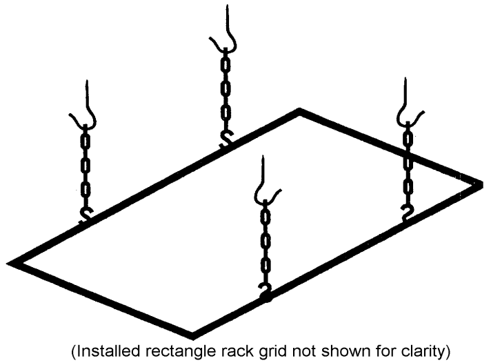
Figure 2 Hook and Chain Assembly
