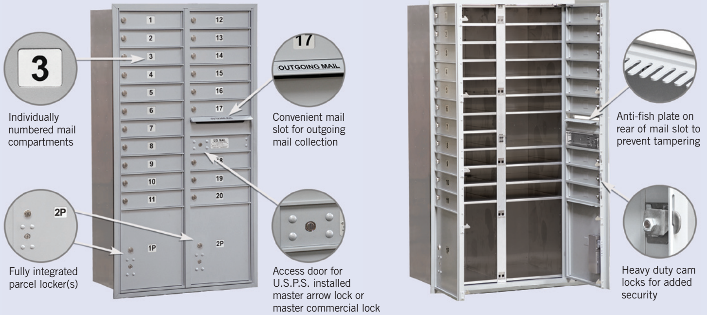
Front views of 3716D-20 front loading unit in aluminum finish displayed
