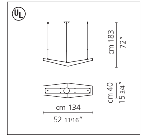
Mouette suspension symmetrical
