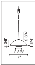
JAS LED DOWN 222 912(bz,mc)/am 222 912(bz,mc)/bl 222 912(bz,mc)/wh
