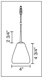
LUCY LED DOWN 222 126(bz,ch,mc) 222 127(bz,ch,mc) 222 128(bz,ch,mc)
