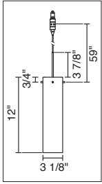
HOUSTON LED DOWN 222 850(bz,ch,mc) 222 851(bz,ch,mc) 222 852(bz,ch,mc) 222 853(bz,ch,mc)
