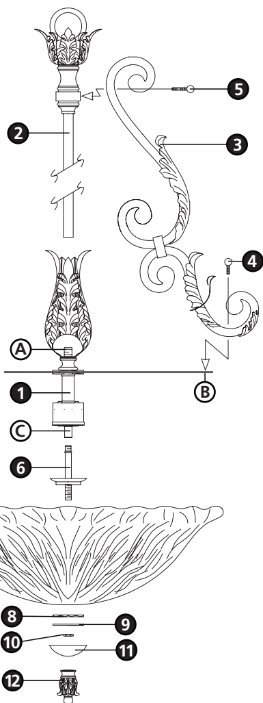
Drawing 1 - Fixture Assembly
