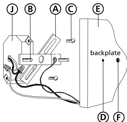
Drawing 3 - Shade Installation
