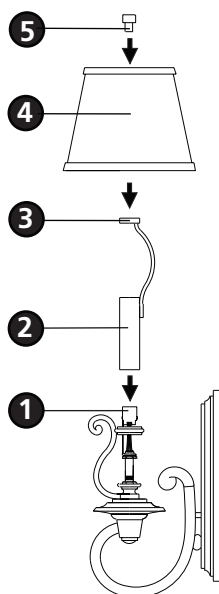
Drawing 3 - Shade Installation
