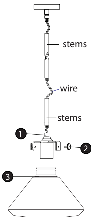
Drawing 3 - Glass Installation
