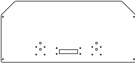
AJI (x1) Backboard
