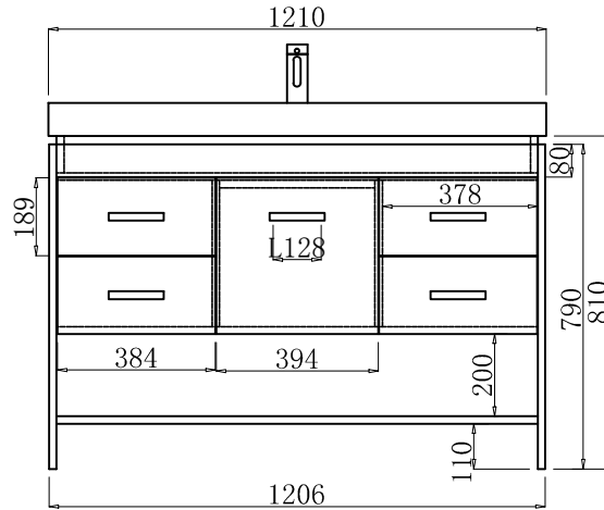
Front view Scale 1:20
