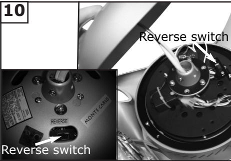
Reverse switch Reverse switch Reverse switch REVERSE MONTE CARLO REVERSE MONTE CARLO Re-place the upper motor housing onto the fan motor. Be sure the holes are all aligned. Note: Align the hole on top housing labeled "REVERSE" with the reverse switch.
