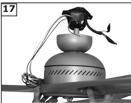
17 Hang the assembled fan from the mounting bracket. Be sure to turn the fan to lock the ridges from the fan and mounting bracket in place.
