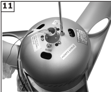
11 Tighten the screws removed from step 5. Tighten securely.
