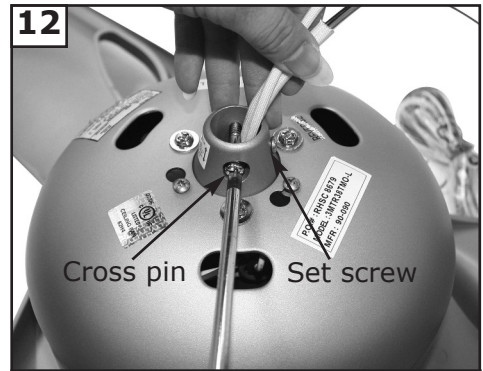
12 Cross pin Set screw Loosen set screw and then remove cross pin from yoke for downrod to slip into yoke. Keep the cross pin for later use.
