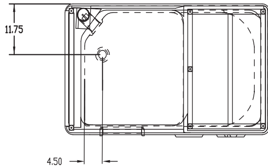
DRAIN TO FRONT WALL
