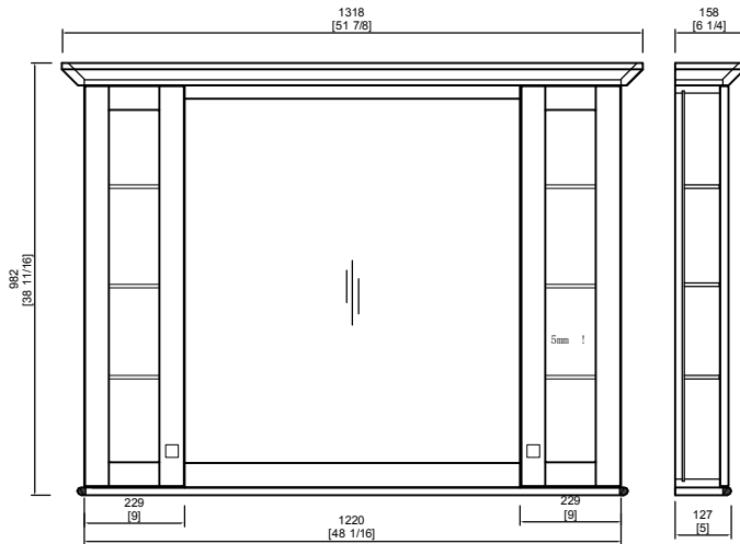
MANHATTAN-M-2130
