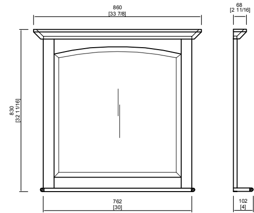
MANHATTAN-M-3030
