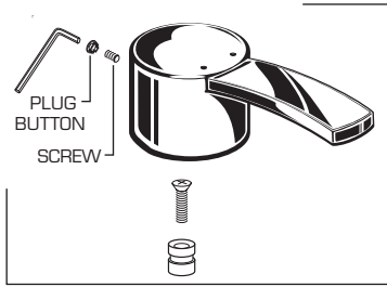
M962828-YYY0A HANDLE KIT
