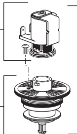
M962664-0070A SOLENOID ASSEMBLY
