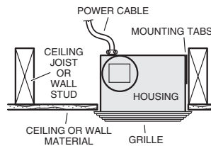
HOUSING MOUNTED DIRECTLY TO CEILING JOIST OR WALL STUD 2x6 (or larger) Discharge parallel to joists or studs.
