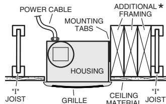
HOUSING MOUNTED IN ANY LOCATION BETWEEN JOISTS Requires additional framing for mounting tabs.
